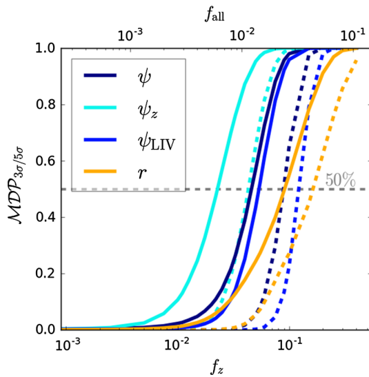
Fig. 5 Detection probability \mathcal{MDP} at 3\sigma (solid) and 5\sigma (dashed lines) for the test statistics \psi , \psi_z , \psi_{LIV} and r as a function of the mean fraction f of GRBs with one associated signal neutrino at t_\nu = t_{\text{GRB}} + 5d \cdot (1+z) . The fraction f_z denotes the fraction of GRBs in the sample with determined redshift z , whereas f_{\text{all}} gives the fraction of the whole sample
