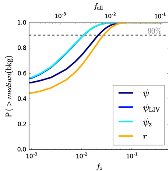
Fig. 6 Probabilities P to measure values of the test statistics above the median value from the background-only realisations as a function of f_z or f_{\text{all}} (as in Fig. 5). The sensitivity is given by the signal fraction f where the curves reach 90% probability (grey dashed line). Note that the curves for \psi_z and \psi_{LIV} lie on top of each other. Probabilities were derived using the ANTARES data from 2007–2012
