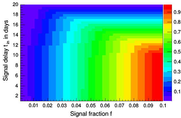
Fig. 4 Detection efficiency (color scale) at the 3\sigma level using the \psi_z test statistic as a function of the signal strength f (see text) and intrinsic time delay at the source for a signal as described in Sect. 4.5
