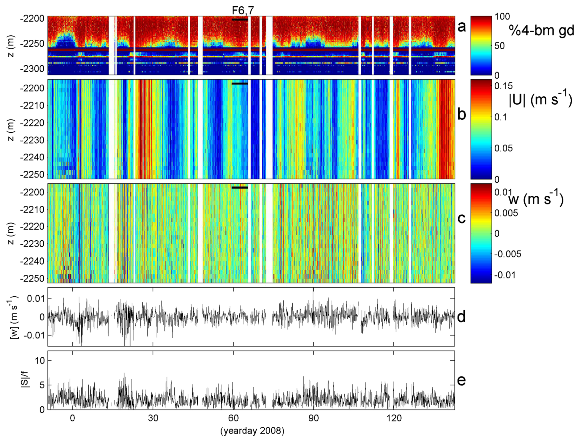
Fig. 4 First 5 months of ANTARES-ADCP depth-time series observed in 2008, plotted every 10th data point. White gaps indicate time lapses >0.5 day. a Percentage of good data when all four beams are working properly, over full range of observations. The range of good data >25\% is approximately between 2,192.5 and 2,252.5 m, except during brief periods like around the beginning of the year (day 0) when it rises to about
