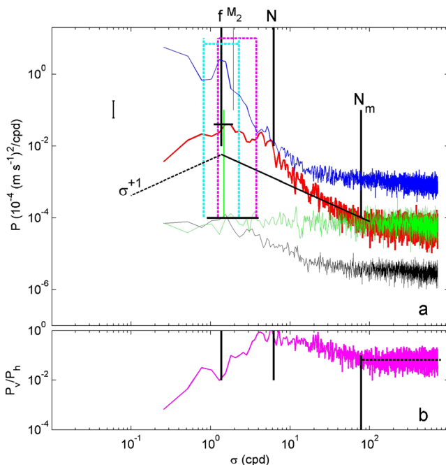
Fig. 9 As Fig. 5 with the same reference slopes and inertio-gravity wave bands, but for different N , N_m for the period of Fig. 8. b The horizontal dashed line indicates the theoretical (manufacturer's) noise level variance ratio
