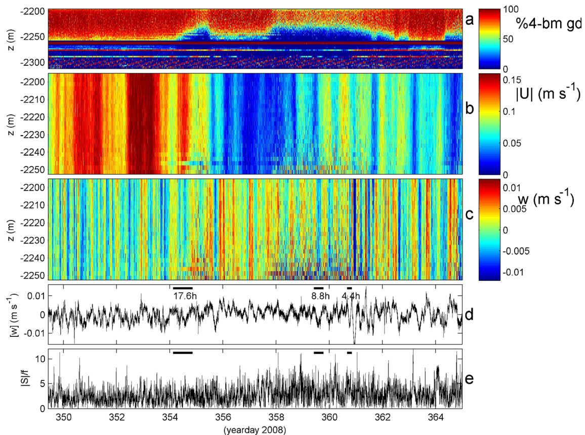
Fig. 8 As Fig. 4, but for 15 days near the end of the year, when sampling rate was highest ( \sim 60 s), artificial time lapses small and far between, and 25-m mean shear relatively high \langle |S| \rangle = 2.9f with incidental values up to |S| \approx 10f
