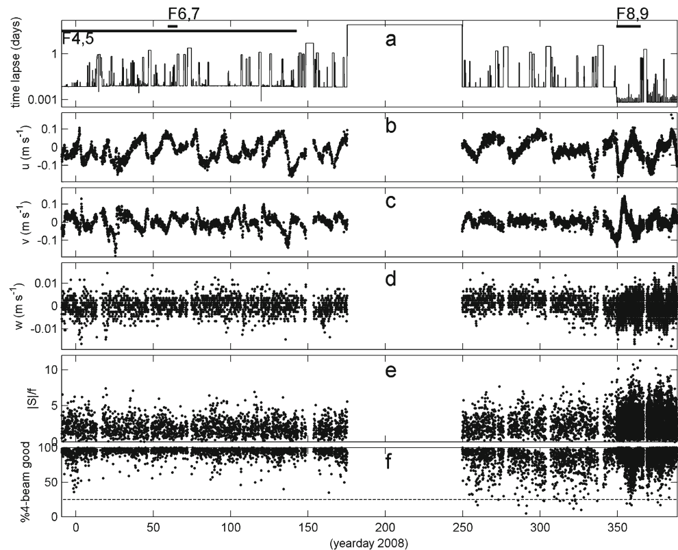
Fig. 3 Yearlong ANTARES–ADCP times series observed at 2,200 m (except for shear in e ) in 2008, plotted every 10th data point. The horizontal bars with Fig. numbers indicate periods shown in more detail in Figs. 4–9. a Time lapse between observations, demonstrating the varying sampling rates and a large data gap in summer. b East–West current component. c North–South current component. d Vertical current component, after removal of overall mean. Note the different vertical scale compared to b , c . e Shear magnitude computed over 25 m, between 2,195 and 2,220 m, in units of local inertial frequency. f Percentage of all four beams providing good data. Lower values are associated with a decrease in reflecting particles. A standard threshold of 25 % is given by the dashed line
