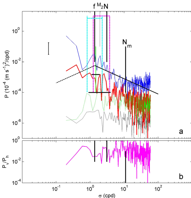
Fig. 7 As Fig. 5 with the same reference slopes and inertio-gravity wave bands, but for different N , N_m for the period of Fig. 6
