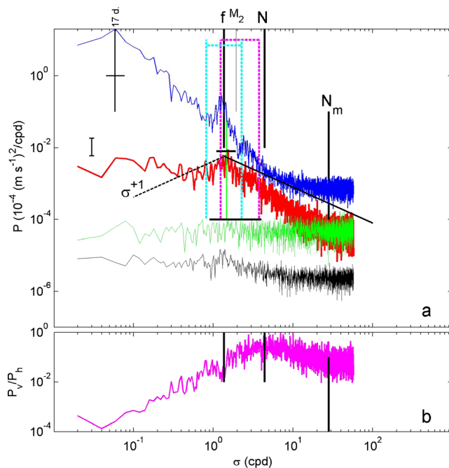
Fig. 5 Power spectra of ADCP data for the period in Fig. 4 in cycles per day. a In red, the vertical current spectrum at 2,210 m is given; in green, the corresponding error velocity. In blue, the corresponding kinetic energy is given, and in black, the 25-m shear spectrum (units 10^{-4} \text{ s}^{-2}/\text{cpd} ). The horizontal black lines indicate levels of maximum \Phi_w(f) and noise (top error velocity, green spectrum). Several frequencies are indicated in the internal wave band by vertical black lines. The vertical green line indicates f_h , the local frequency for horizontal Coriolis parameter. Two special frequencies are the following: the frequency where the spectrum \Phi_w deviates from the \sigma^{-1} -slope is labelled “N”, the frequency where \Phi_w reaches noise level is labelled “ N_m ”. For reference, one semidiurnal tidal frequency ( M_2 ) is given, two spectral slopes and two inertio-gravity wave bands, for N=1f (light-blue lines) and for N=2.5f (purple). The vertical black bar indicates the 95 % confidence limits. b Ratio of vertical (red spectrum in a ) over horizontal (blue spectrum in a ) current variance
