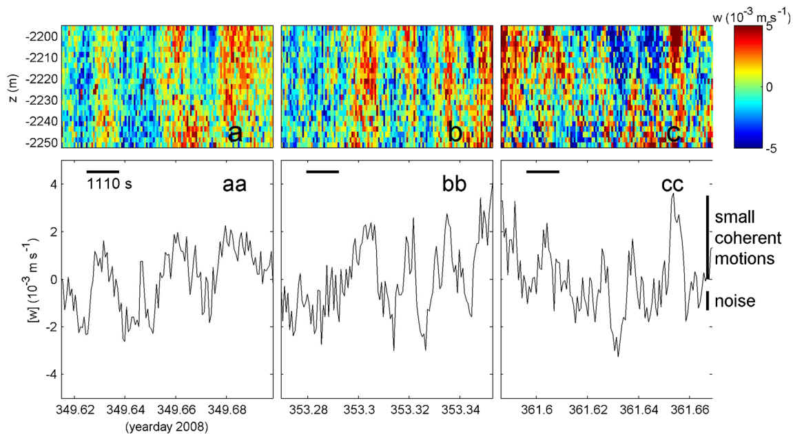
Fig. 10 Three 2-h periods of vertical currents, with respect to their local time mean, from Fig. 8c (a–c) and Fig. 8d (aa–cc: here, vertical average is over full range of 60 m in a–c); the shortest period T_{Nm}=1,110 s. Bars to
