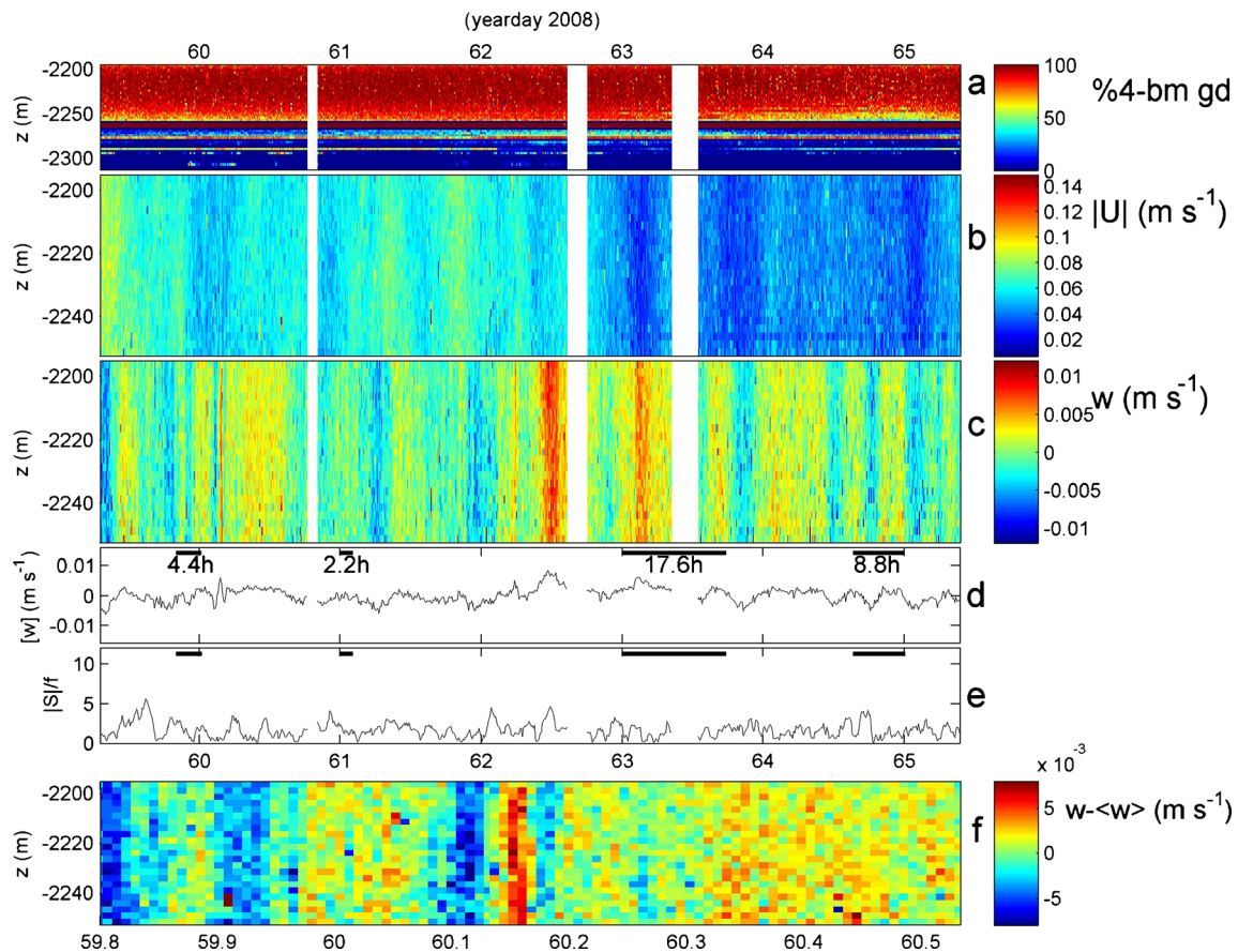
Fig. 6 As Fig. 4, but for 6 days when time-mean 25-m shear was low, \langle |S| \rangle = 1.7f . Here, white gaps indicate time lapses >1.5 h. The local inertial period ( T_f = 2\pi/f \approx 17.6 h) is indicated, as well as 0.5T_f , 0.25T_f , 0.125T_f (corresponding to frequencies 2f , 4f , 8f , respectively). In f , a
