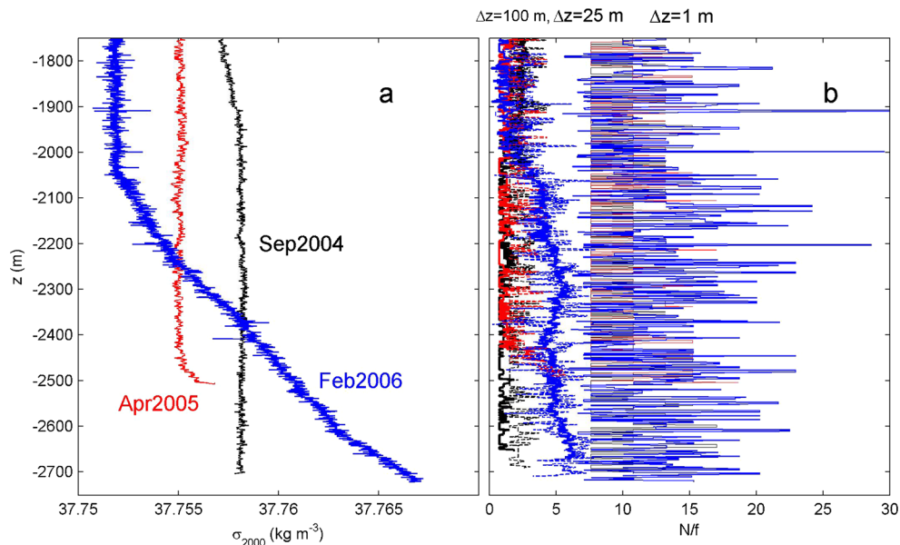
Fig. 1 CTD-parameter profiles as a function of depth from central West Mediterranean ( 40^{\circ} N, 6^{\circ} E), measured during three campaigns “Gyroskop” outside ANTARES. a Density anomaly ( -1,000 \text{ kg m}^{-3} ), referenced to 2,000 m. b Buoyancy frequency in units of inertial frequency computed over \Delta z=1 \text{ m} intervals ( thin lines ), over \Delta z=25 \text{ m} ( dashed lines ), and over \Delta z=100 \text{ m} ( thick lines ), positive definite values only. The
